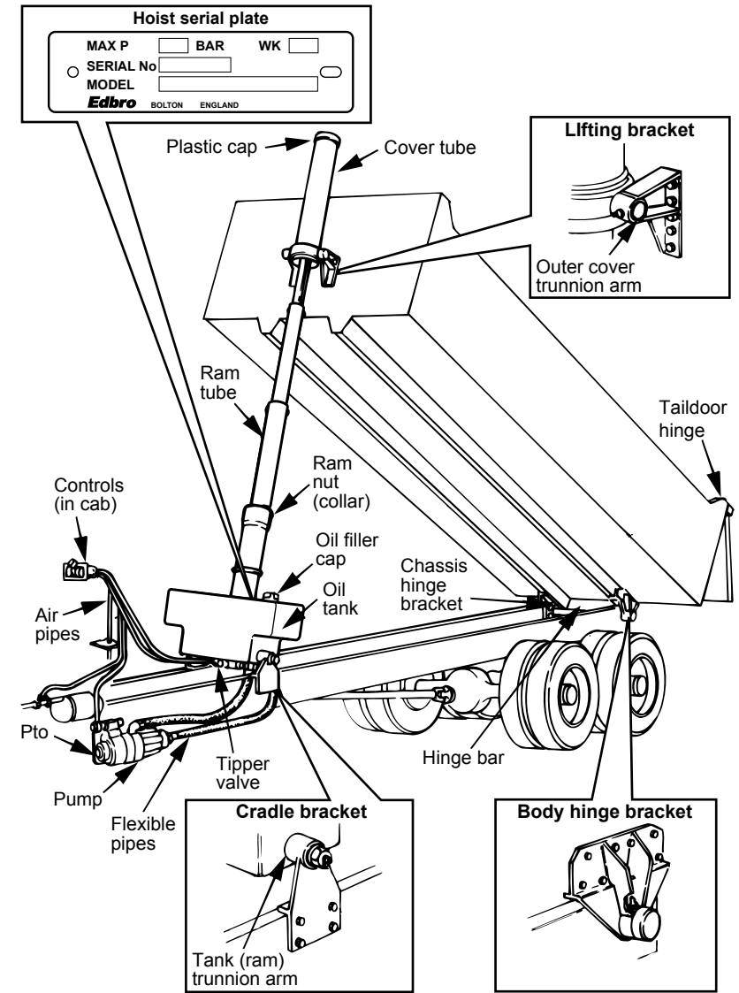
CX Combined ram and tank hoist
