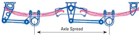
Featuring 2 leaf spring
