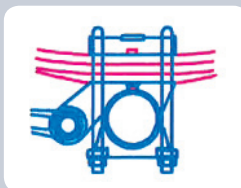
Overslung inverted
