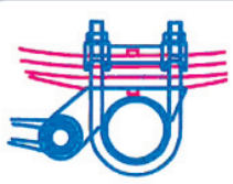
Overslung conventional
